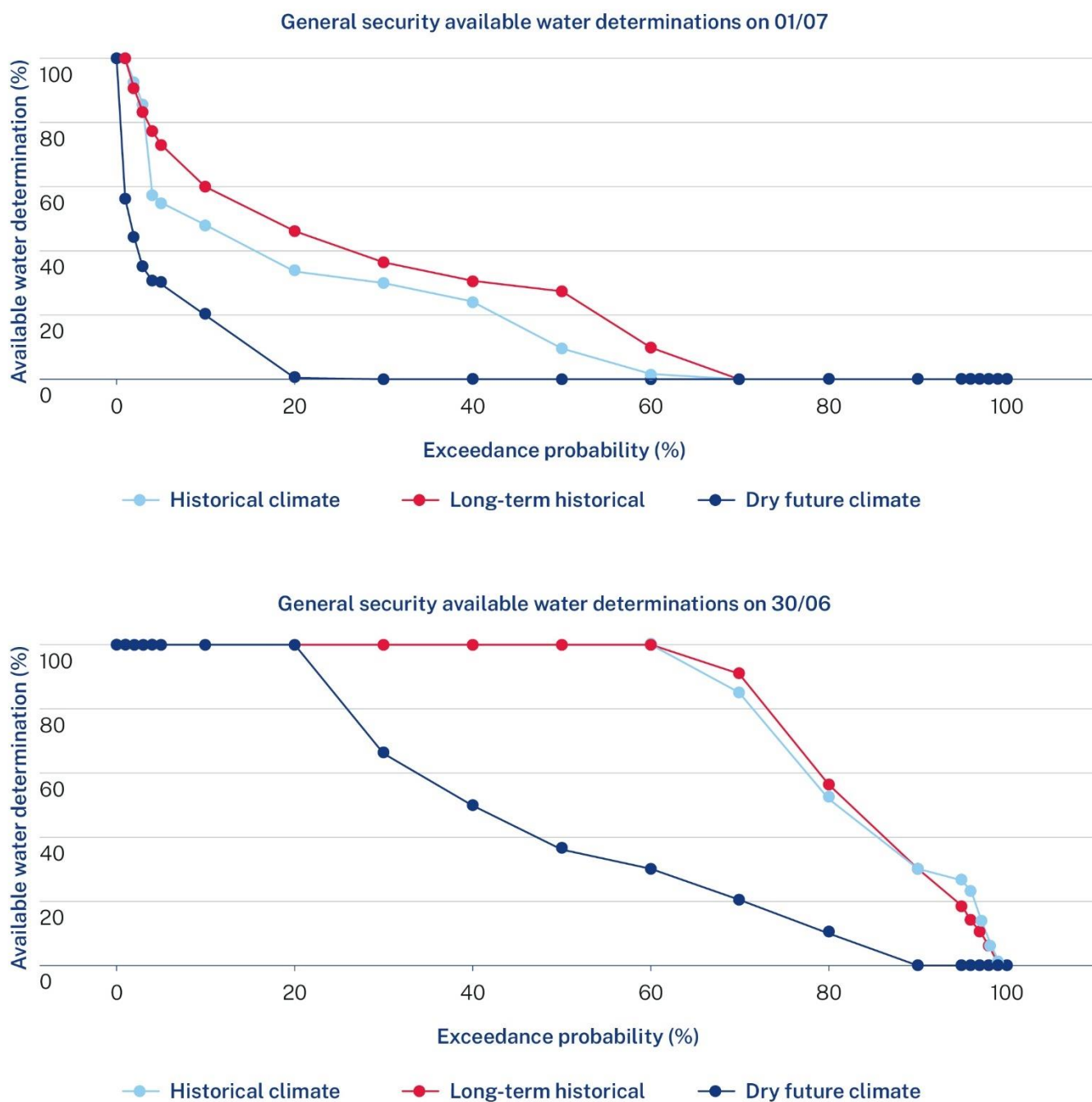
Figure 9 Impact of climate scenario on NSW Murray general security available water determinations for 1 July (top) and 30 June (bottom)
