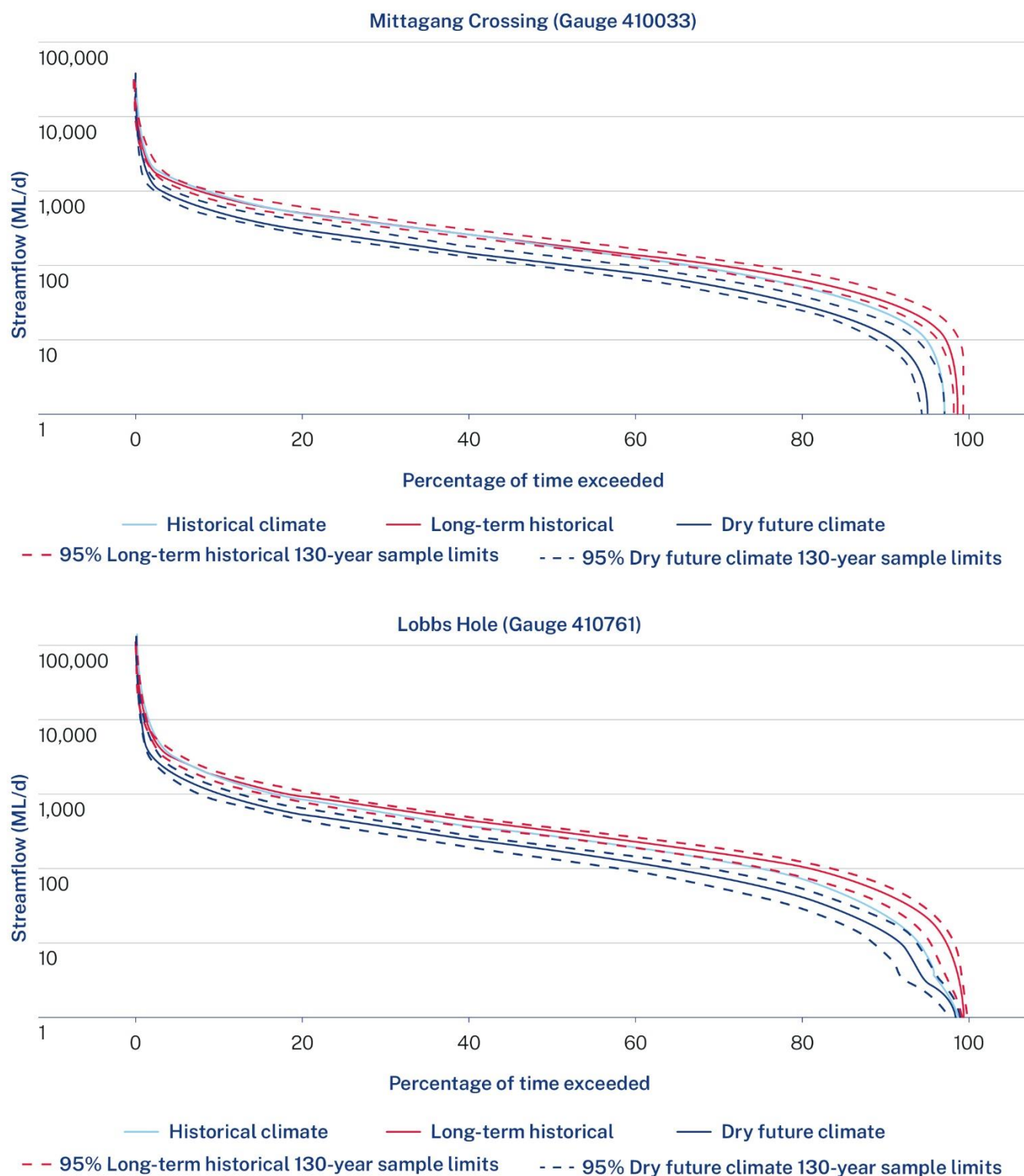
Figure 16 Impact of climate scenario on flow duration in the Murrumbidgee River at Mittagang Crossing (top) and Lobbs Hole, ACT (bottom)
