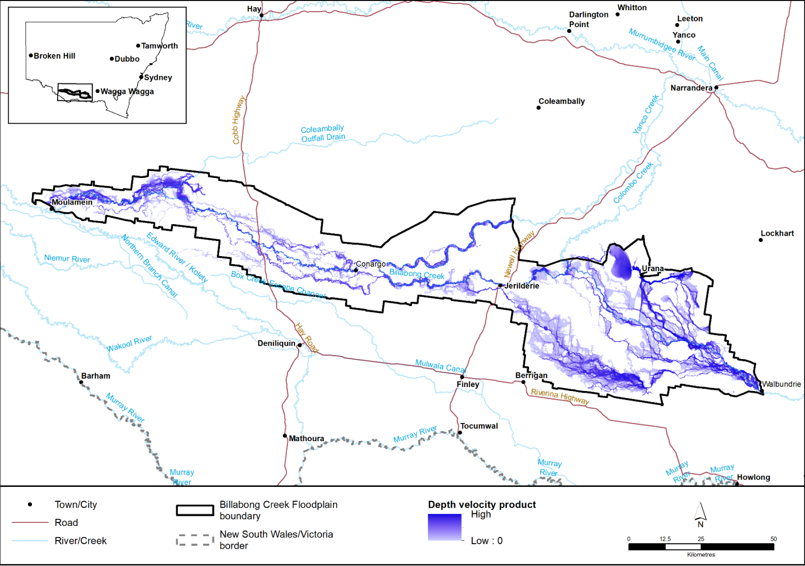
Figure 5: Hydraulic modelling results (depth-velocity product) map from all 3 models for the large design flood event (October to November 2022 – 5% AEP at the Billabong Creek at Jerilderie gauge)
