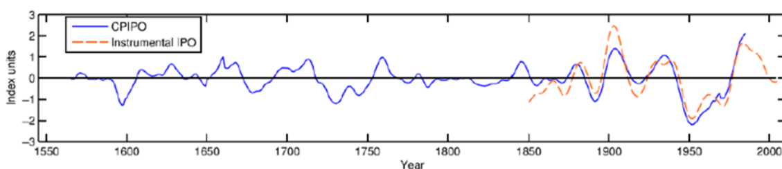
Figure 8. Comparison of the instrumental IPO time series to the combined paleo IPO time series, 1550 to 2000 CE
