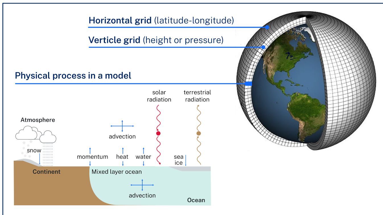
Figure 12. Simple schematic of a general circulation model
