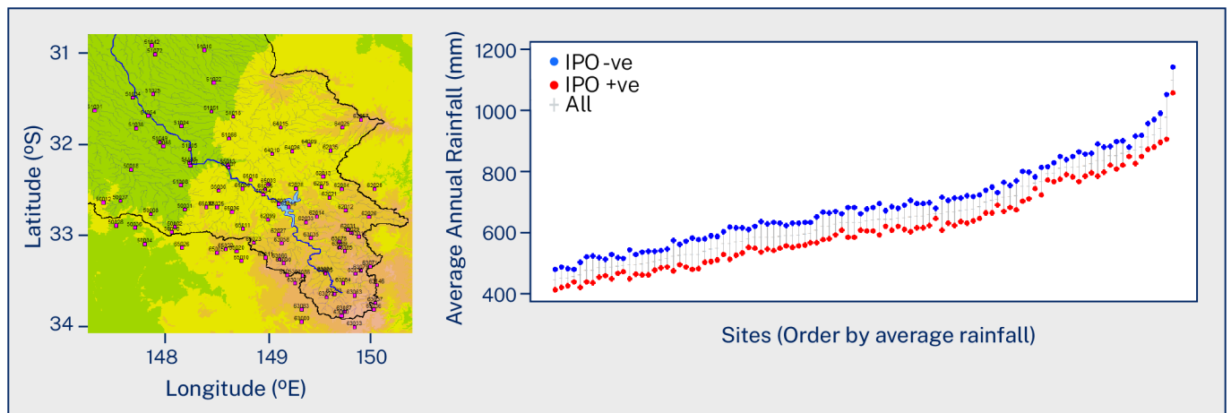
Figure 7. Rainfall sites in Macquarie catchment (left) with mean annual rainfall reported by IPO phase (right panel)
