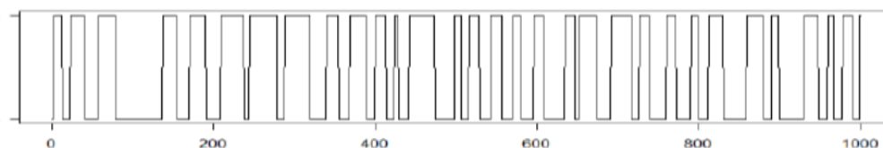
Figure 10. Generated IPO phases for a 1,000-year sample
